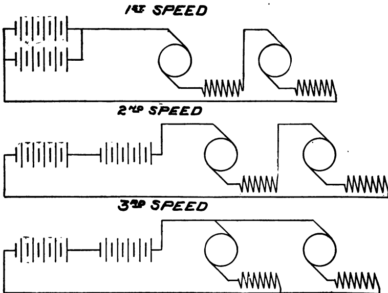
FIG. 906.—Diagram of a Two-Battery-Unit, Two-Motor Circuit, showing combinations for three speeds. The first speed is obtained with the battery units in multiple , and the motors in series ; the second, with the battery units in series , and the motors in series ; the third, with the battery units in series , and the motors in multiple .
